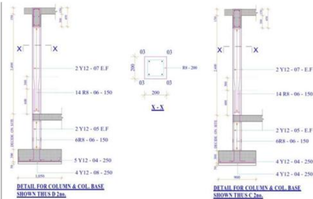
1:1 COLUMN DETAILS
